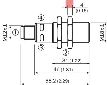
Dimensional drawing UM18-2xxxxx1
