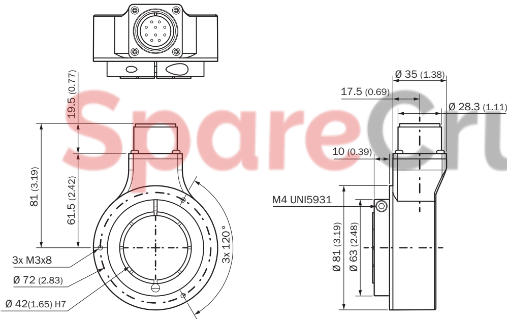
Dimensional drawing Bore hole size 42 mm, MS male connector
