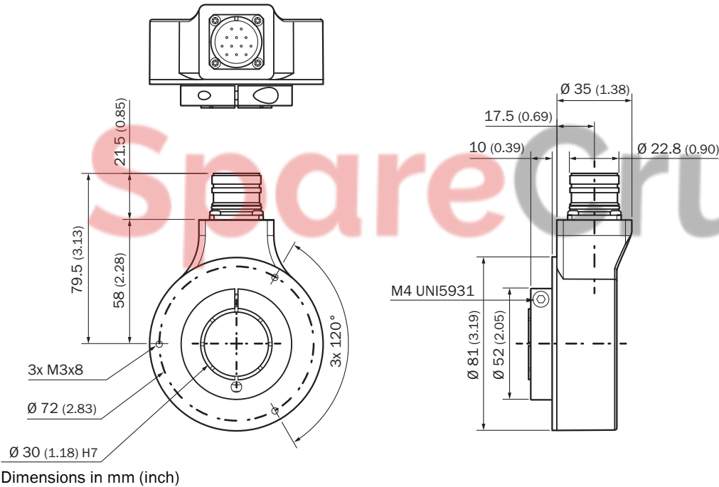
Dimensional drawing Bore hole size 30 mm, M23 male connector
