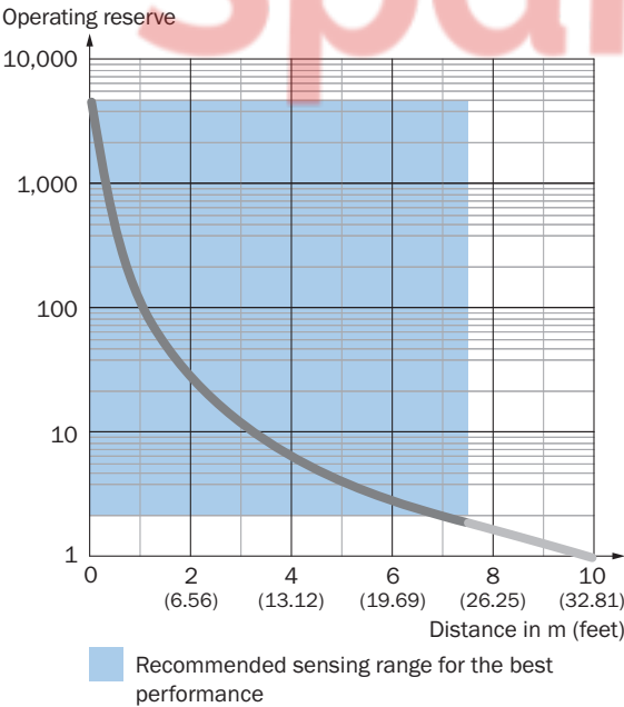
Characteristic curve
